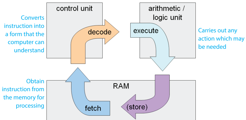
Fig. 2.1: Fetch-Execute Cycle
