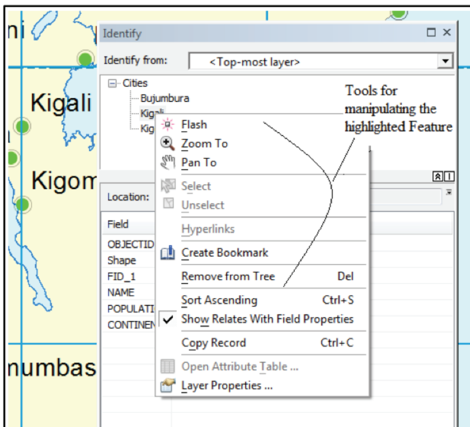
Fig. 7.22: Menu showing more options for a Feature
