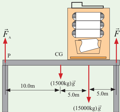
Figure 3.15: Indicating forces developed in a beam
