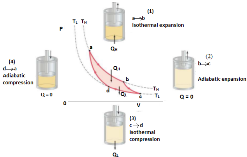
Figure 10.13: Carnot Cycle
