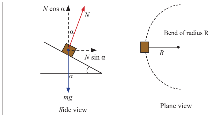
Figure 7.15: Rounding a bend
