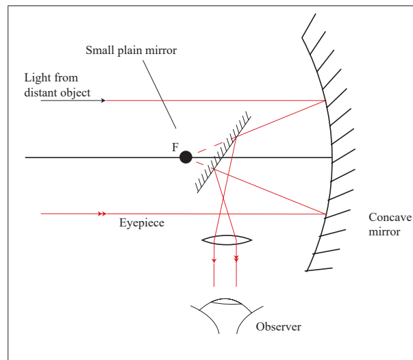
Figure 2.29: The Newtonian reflecting telescope
