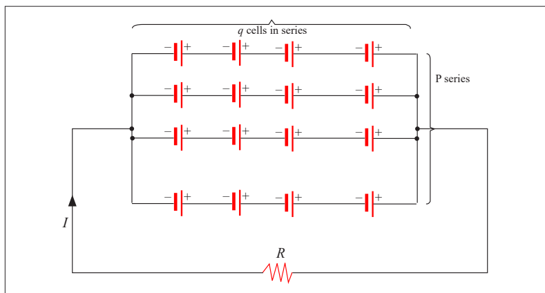
Figure 5.21: Mixing of a series and parallel combination
