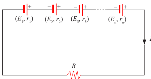
Figure 5.15: Cells combined in series
