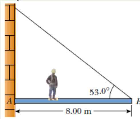
Fig.3. 21 A uniform beam supported by a cable. A person walks outward on the beam
