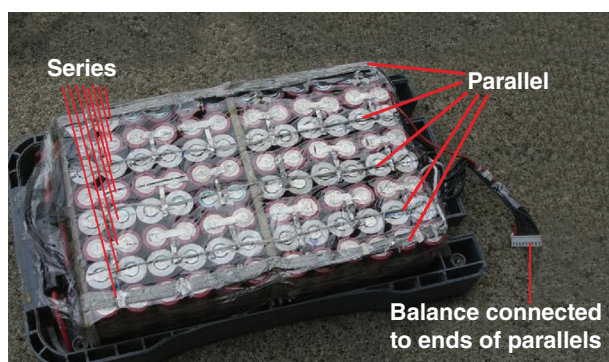
Figure 5.22: Identical series combined in parallel
