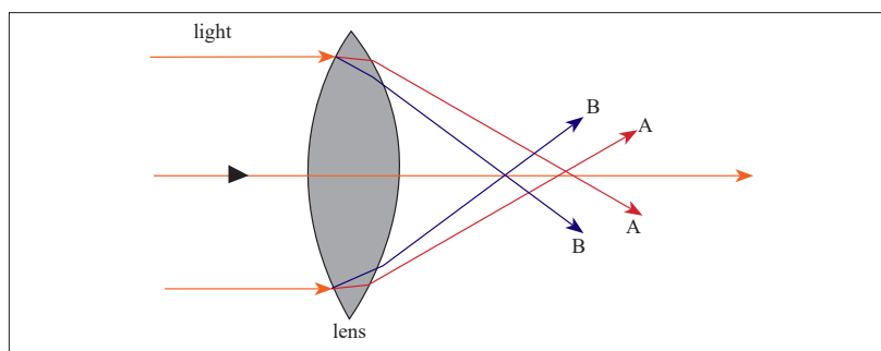
Figure 1.31: Chromatic aberration
