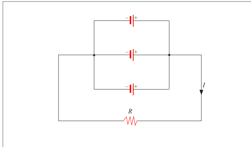
Figure 5.19: Identical cells combined in parallel
