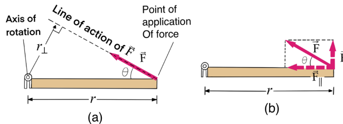
Figure 3.1: Lever arm
