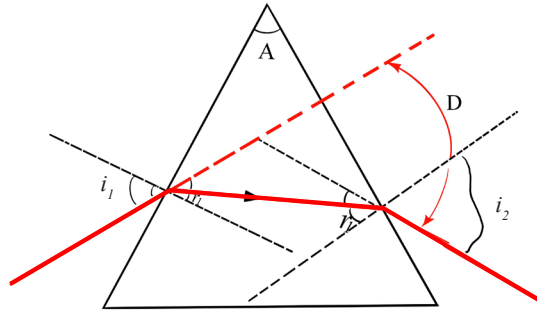
Figure 1.43: Minimum deviation
