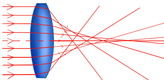
Figure 1.30: Spherical aberration
