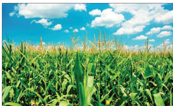
Figure 6.6: Biological material
