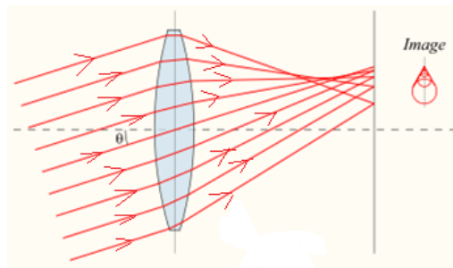
Fig.1. 31 Coma aberration
