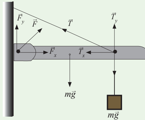
Figure 3.19: Showing forces acting on a bar fixed at one point with a mass connected at one point
