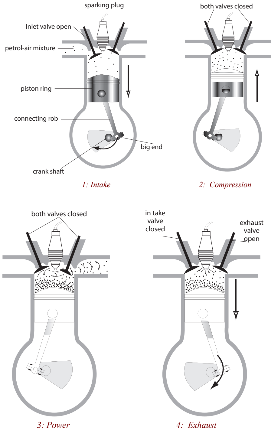
Fig 10.16: For stroke-cycle interval combustion
