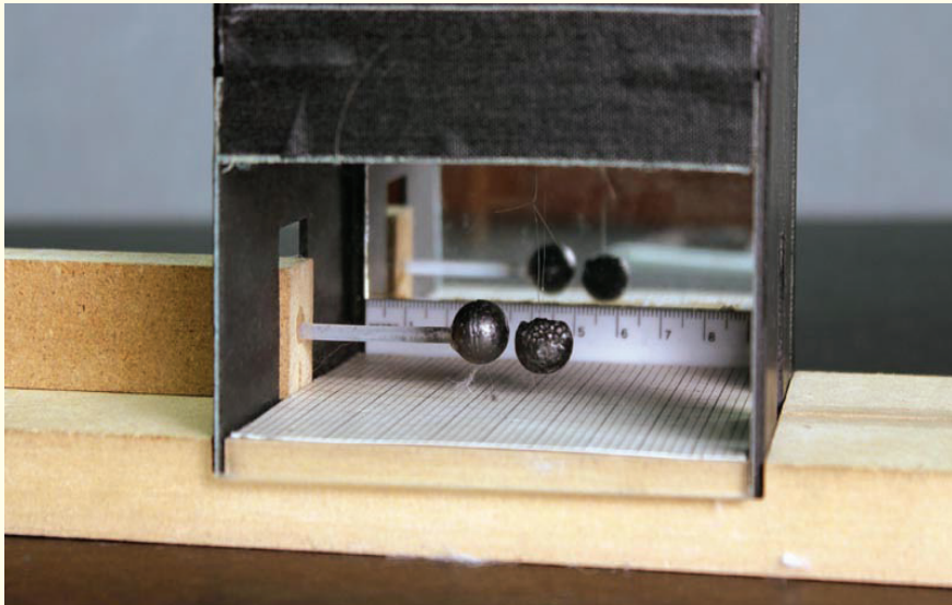
Figure 9.2: Coulomb's apparatus
