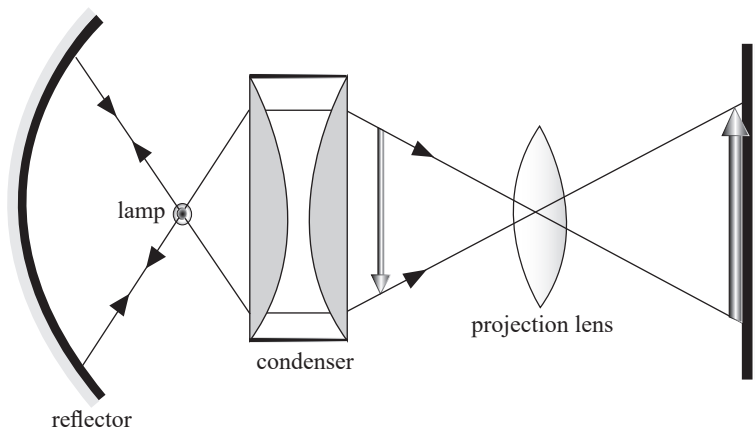
Figure 2.13: Projector
