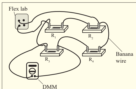
Figure 5.26: Voltage measurements
