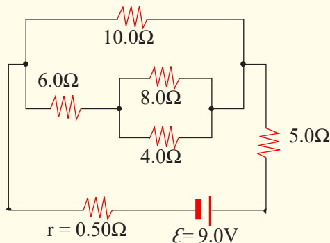
Figure 5.25: Related circuit to question 4
