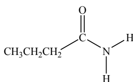
butanamide
