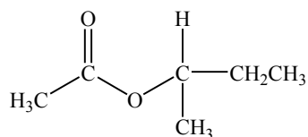
1-methylpropylethanoate
