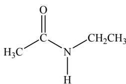
N-ethylethanamide
