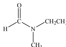
N-ethyl-N-methylmethanamide
