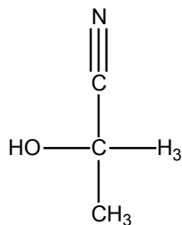
2-hydroxy-2-methylpropanenitrile
