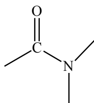
Amide group
