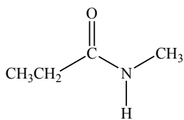
N-methylpropanamide
