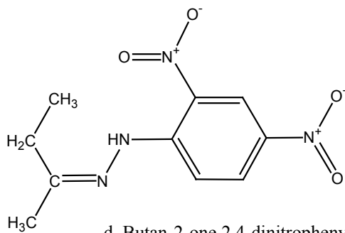
d. Butan-2-one 2,4-dinitrophenylhydrazone
