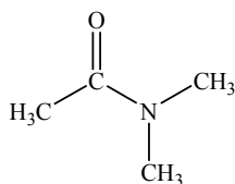
N,N-dimethylethanamide
