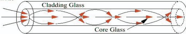
Figure 2. 5: Multimode Optical Fiber
