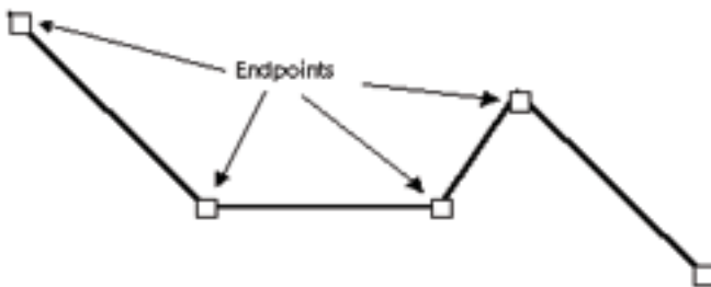
Figure 12.60 Polyline
