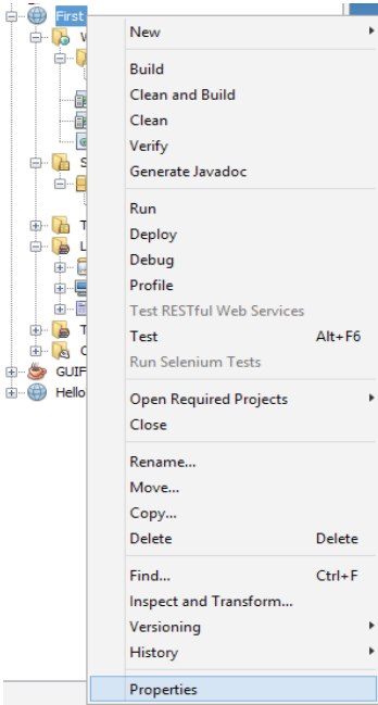
Figure 11.225: Project properties
