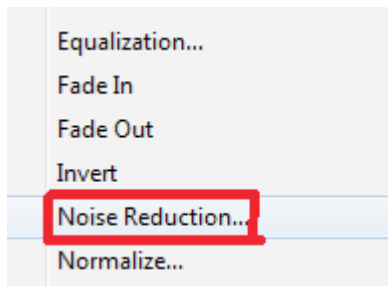
Figure13.26: Noise reduction
