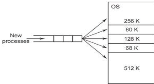
Figure 9.6.: Single queue
