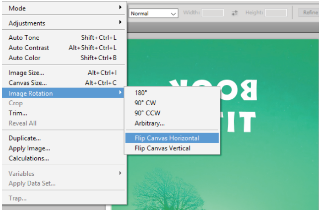
Figure 12.55 Rotate image
