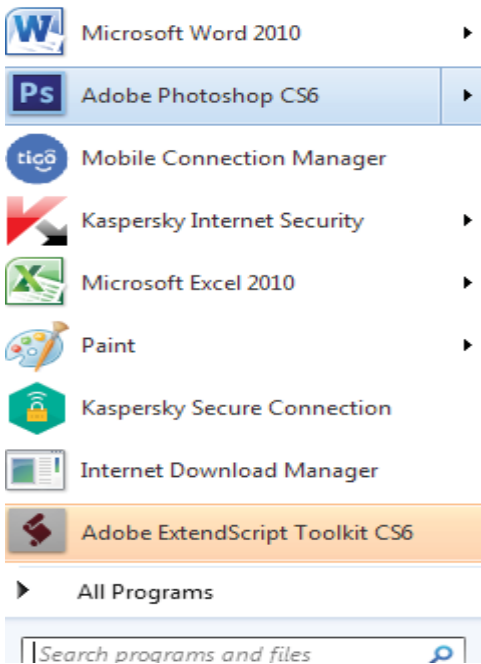
Figure 12.28 Launch Photoshop
