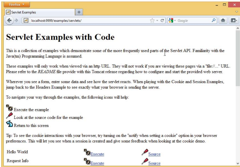
Figure 11. 10: Servlet examples
