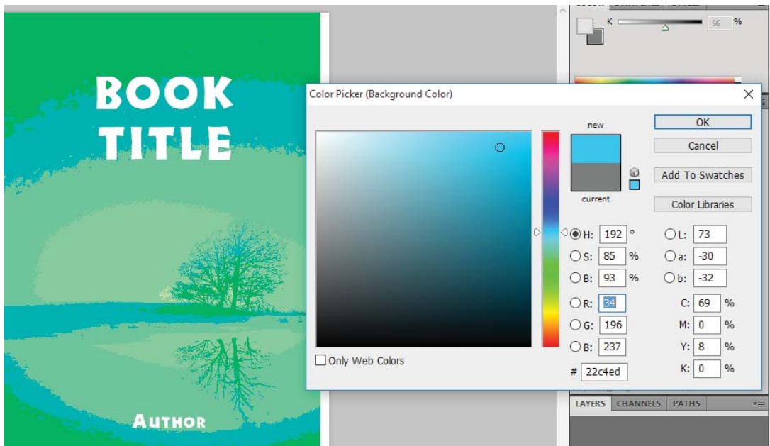
Figure 12.38 coloured image
