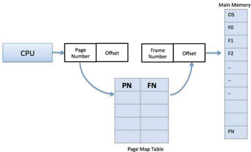
Figure 9.14.: Mapping
