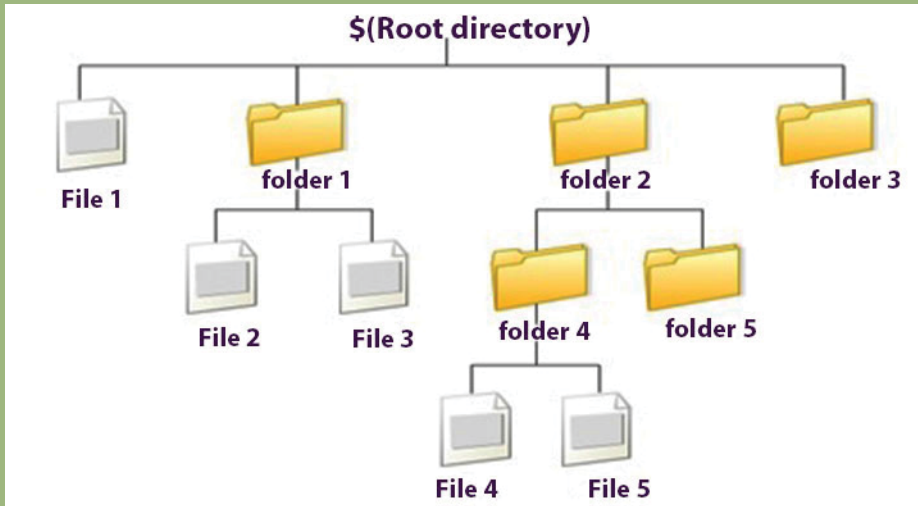
Figure 8.2: File Hierarchy
