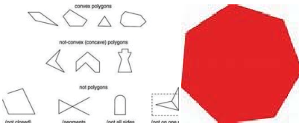
Figure 12.61 Polygon
