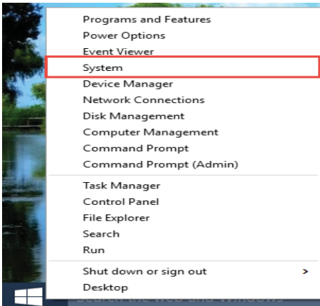
Figure 3.14: Selecting system
