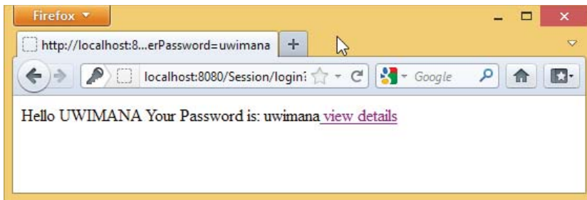
Figure 11.43: Login page
