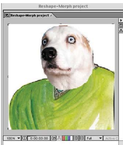
Figure 13.66: Morphed image
