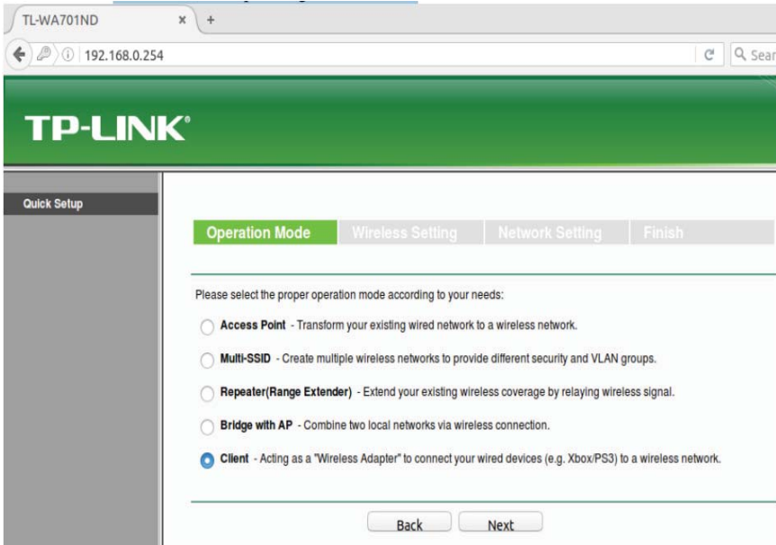
Figure 2.26: Operation mode
