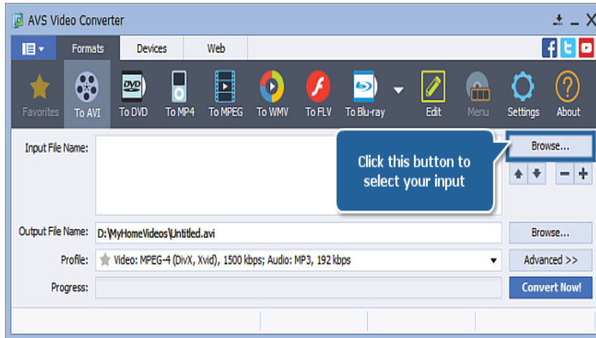
Figure 13.48: Video input
