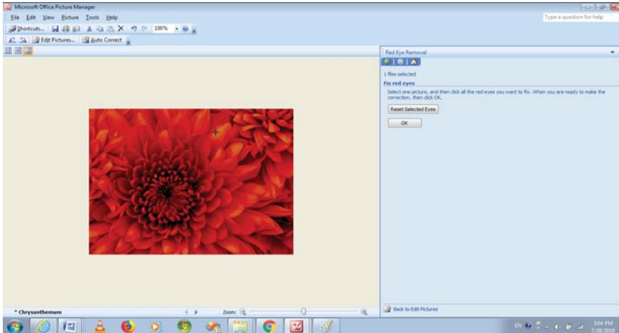
Figure 12.25 Red-eye removal
