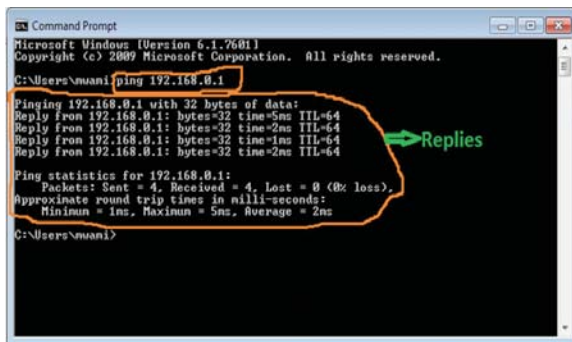
Figure 3.12: Verifying connection
