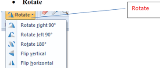
Figure 12.20 Rotate
