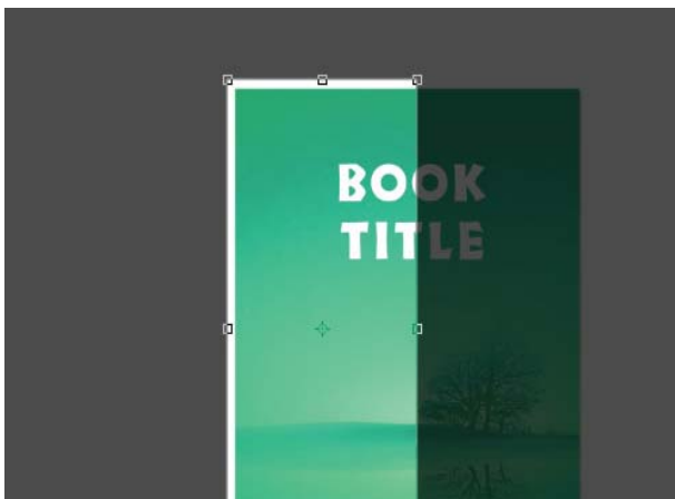
Figure 12.54 crop
