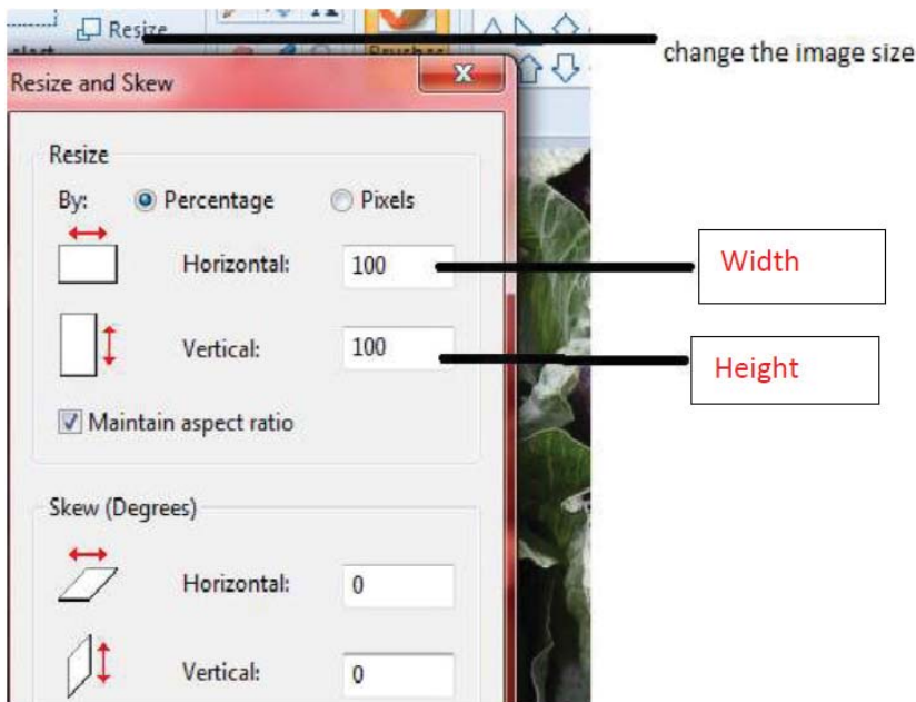
Figure 12.18 resizing image
