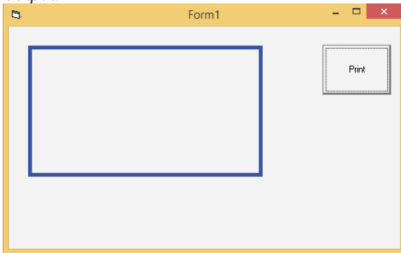
Figure 14: Rectangle
