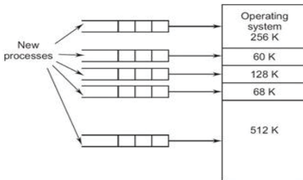
Figure 9.5: Multiple queues
