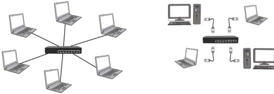
Figure 3.6: Connected devices
