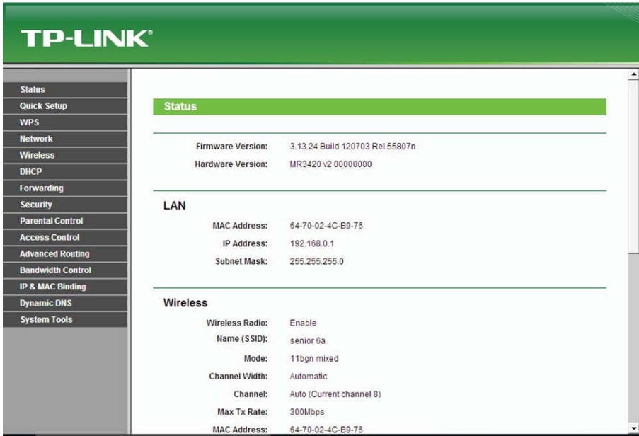
Figure3.22: Default dashboard
