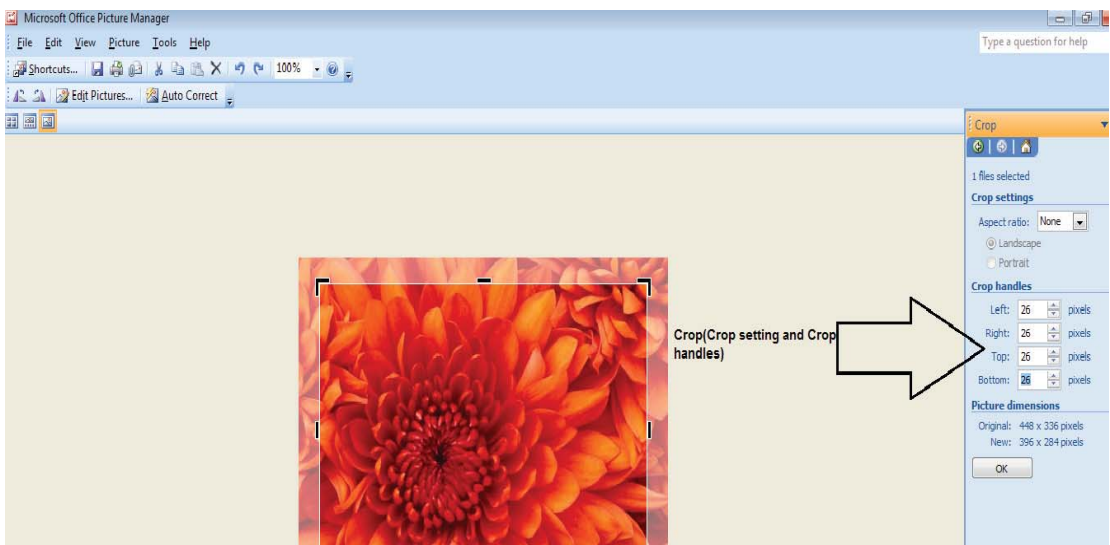
Figure 12.24 Crop
