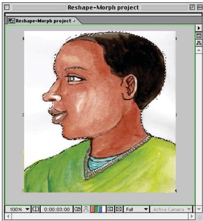
Figure 13.58: Creating mask
