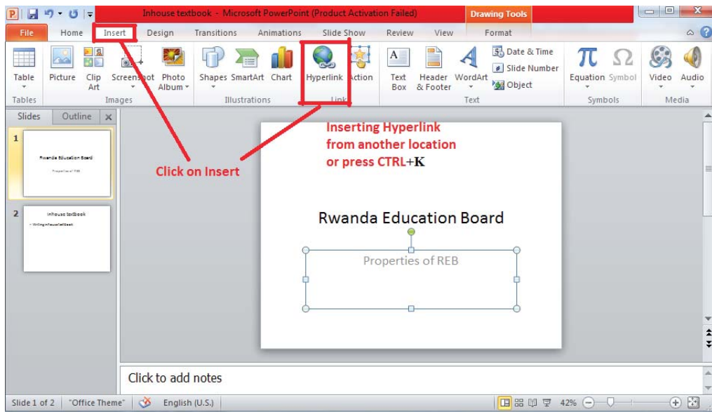
Figure 13.4: Hyperlink Location
