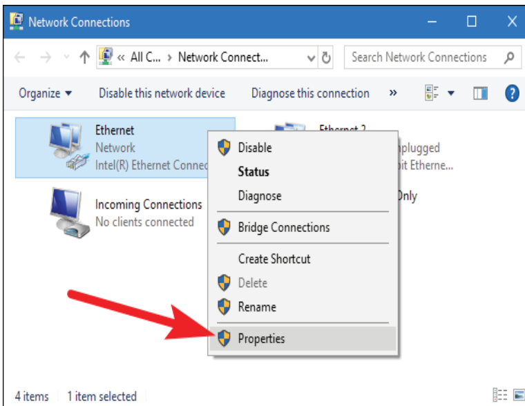
Figure 3.10: Viewing properties
