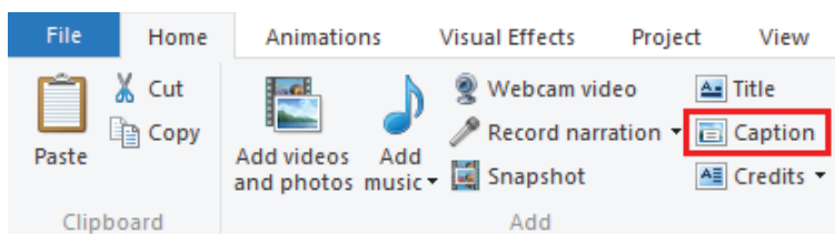
Figure 13.54: Adding caption
