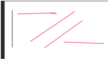
Figure 12.49 Lines
