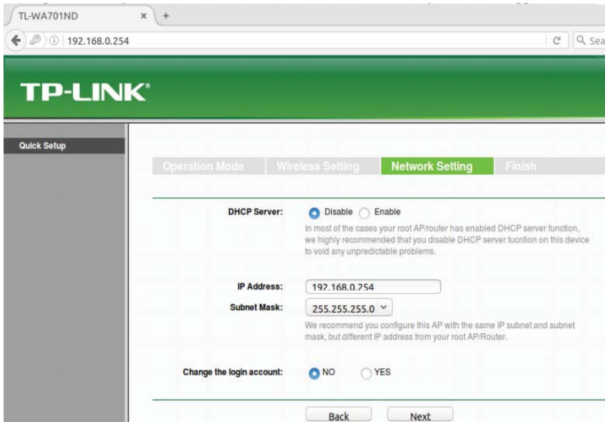
Figure 2.30: Network settings
