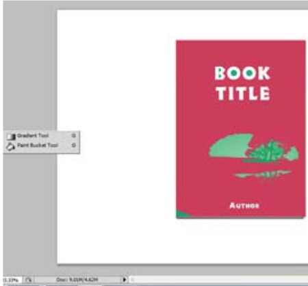
Figure 12.43 paint bucket
