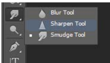
Figure 12.45 sharpen
