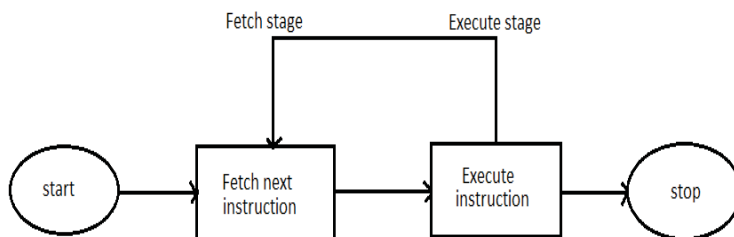
Figure 7.2. Process execution
