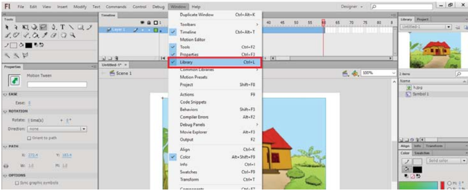
Figure 13.43: Selecting Library
