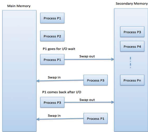
Figure 9.10: Swapping Mechanism
