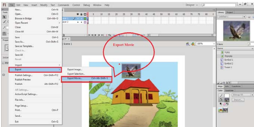
Figure 13.47: Export movie
