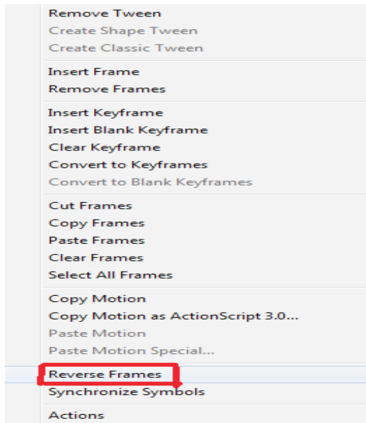
Figure 13.39: Reversing frames
