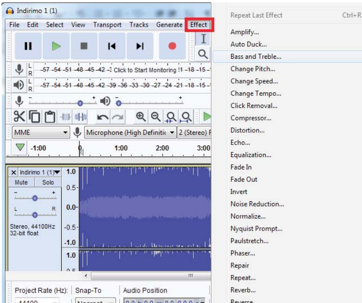
Figure 13.19: Opening Effect
