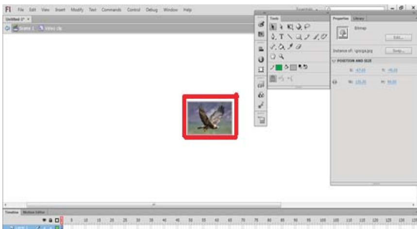
Figure 13.35: Importing image
