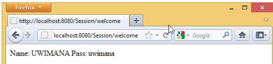
Figure 11.44: Login details
