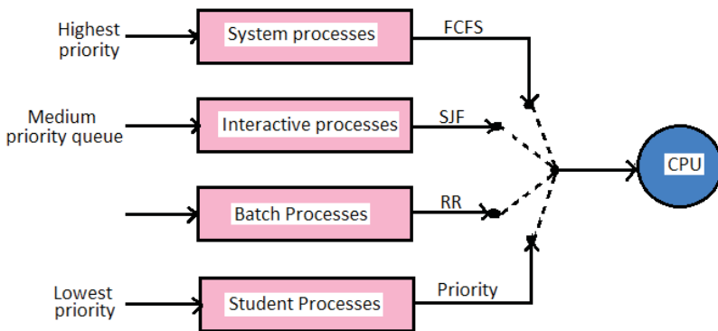
Figure 7.15: Multilevel Queue Scheduling
