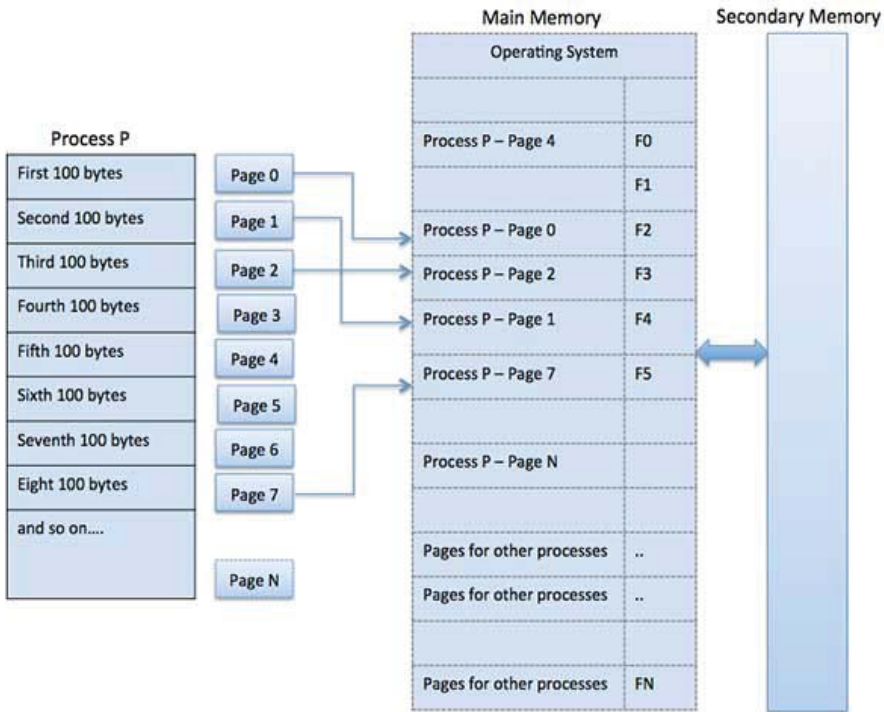
Figure 9.13: Paging Source: https://www.tutorialspoint.com
