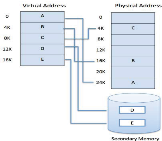
Figure 9.12.: Demand Paging Source: https://www.tutorialspoint.com
