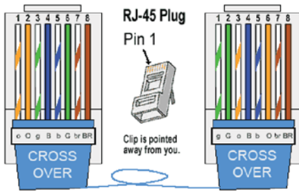
Figure 3.3: Crossover cable
