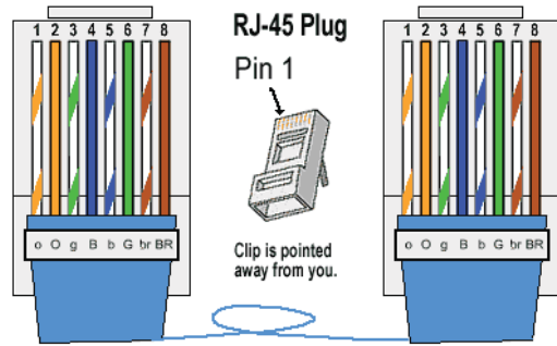
Figure 3.4: Strait through cable
