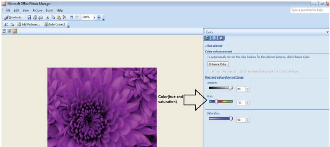
Figure 12.23 Colour
