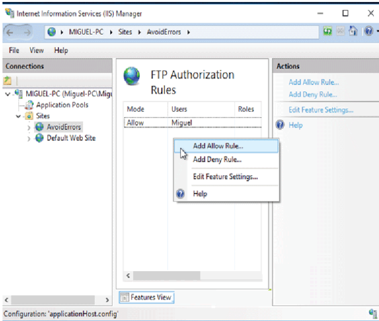
Figure 3.3.13: Allowing rule
