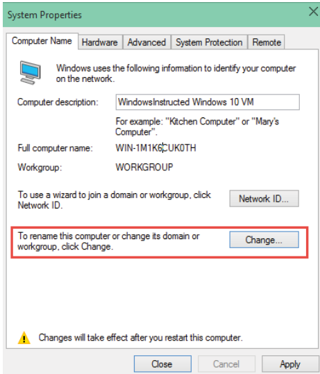
Figure 3.16: Select Change
