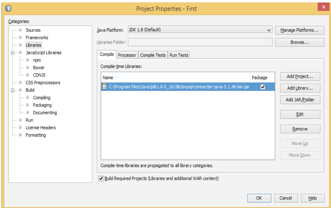
Figure 11. 23: Project libraries
