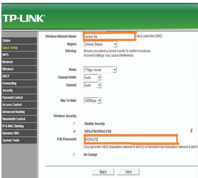
Figure3.25: Network authentication
