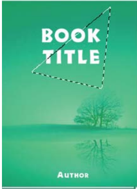
Figure 12.52 polygon lasso
