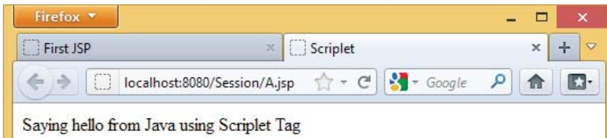
Figure 11.51: Scriptlet
