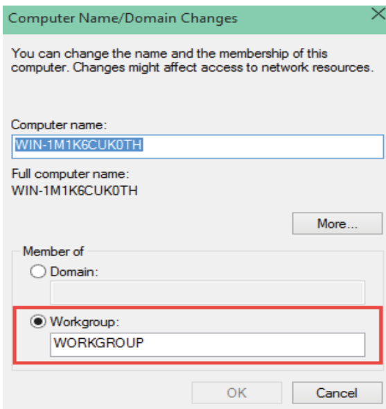
Figure 3.17: Select workgroup
