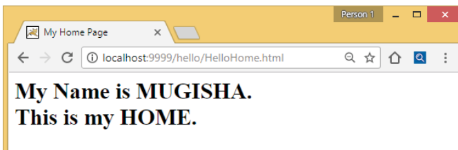
Figure 11. 26: Welcome page
