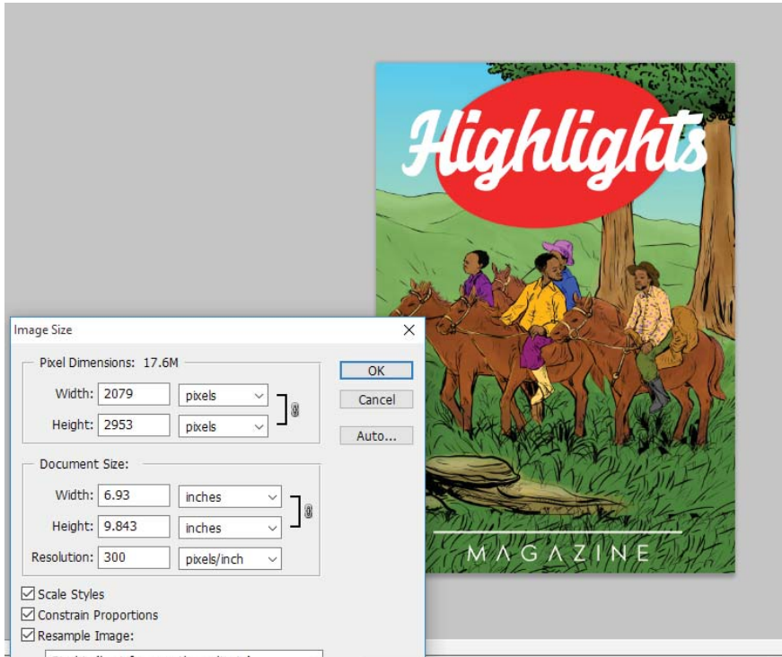
Figure 12.30 image size
