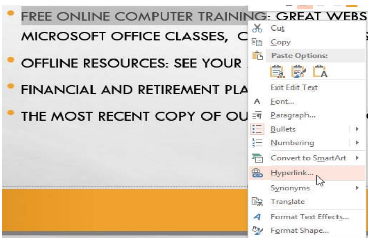
Figure 13.1: Image location
