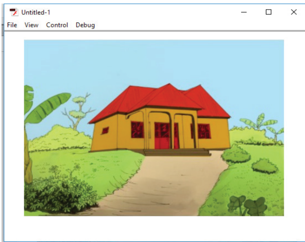
Figure 13.42: Displaying animation
