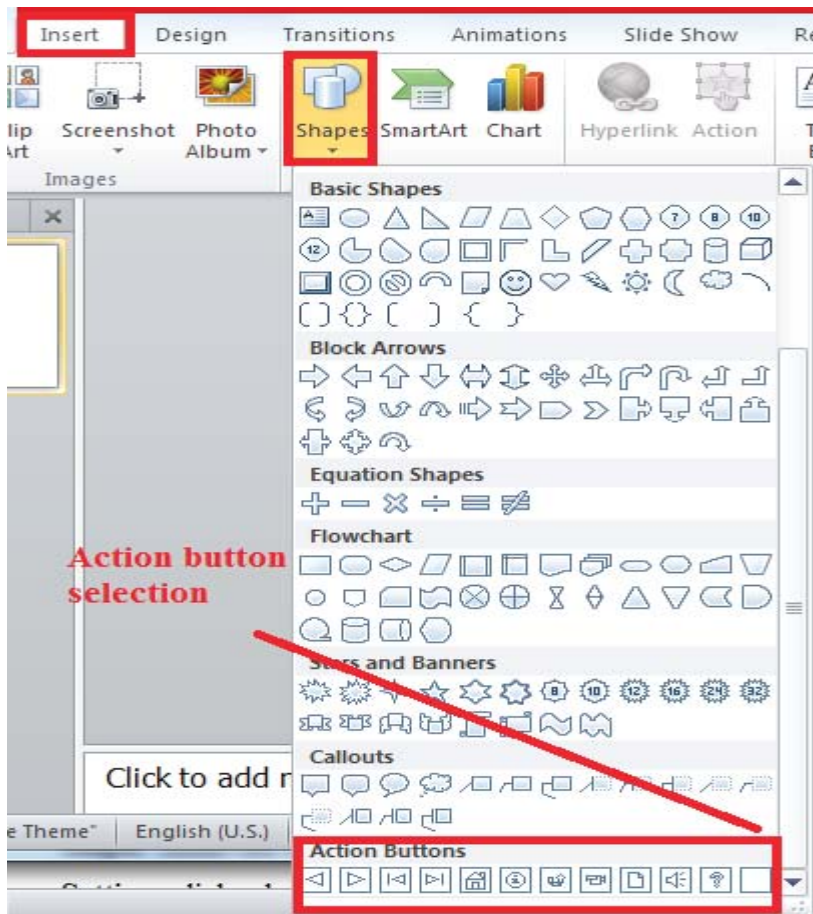
Figure 13.10: Shape command
