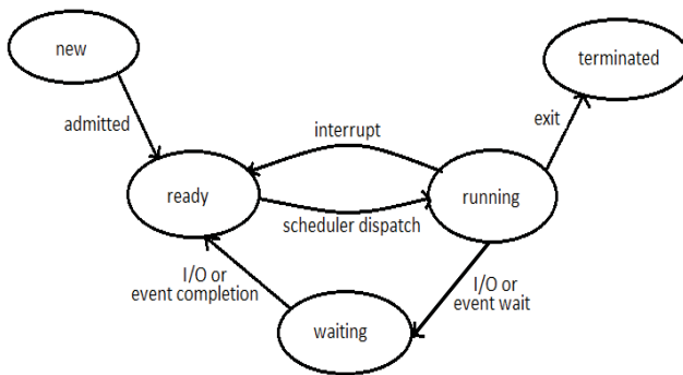
Figure 7.3: process states diagram
