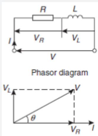
Figure 1.8: R-L series circuit
